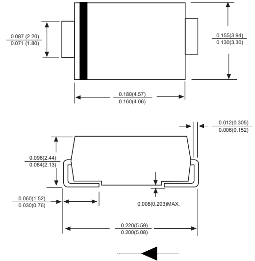
SMB/DO-214AA
